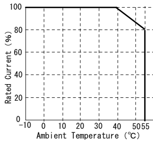
Ambient Temperature - Allowable Current Characteristic
