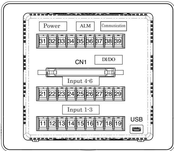
[Terminal Block Array]
